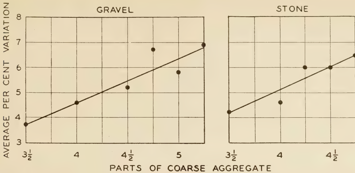
FIGURE 31.—UNIFORMITY OF CONCRETE: AVERAGE PERCENTAGE VARIATION OF MODULUS OF RUPTURE OF INDIVIDUAL SLABS FROM AVERAGE MODULUS OF RUPTURE FOR THE SECTION OF 4 SLABS
